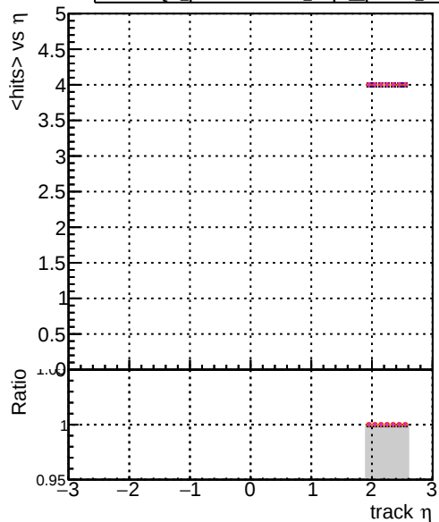
DQM original step2_pt1to20_eta2p0to2p5 DQM mkrFit_step2_pt1to20_eta2p0to2p5 DQM angle_step2_pt1to20_eta2p0to2p5 DQM fast_step2_pt1to20_eta2p0to2p5 DQM pixelCPEGeneric_step2_pt1to20_eta2p0to2p5
