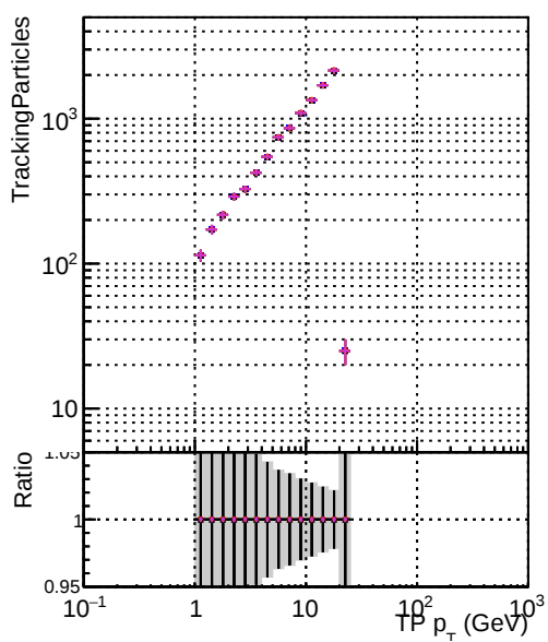
— DQM original step2 pt1to20 eta2p0to2p5 — DQM mkFit step2 pt1to20 eta2p0to2p5 — DQM angle step2 pt1to20 eta2p0to2p5 — DQM fast step2 pt1to20 eta2p0to2p5 — DQM pixelCPEGeneric step2 pt1to20 eta2p0to2p5
