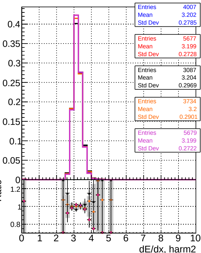
— DQM original step2 pt1to20 eta2p0to2p5 — DQM mkFit step2 pt1to20 eta2p0to2p5 — DQM angle step2 pt1to20 eta2p0to2p5 — DQM fast step2 pt1to20 eta2p0to2p5 — DQM pixelCPEGeneric step2 pt1to20 eta2p0to2p5
