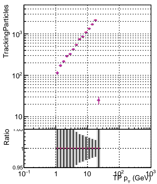
— DQM original step2 pt1to20 eta2p0to2p5 — DQM mkrfit_step2 pt1to20 eta2p0to2p5 — DQM angle_step2 pt1to20 eta2p0to2p5 — DQM fast_step2 pt1to20 eta2p0to2p5 — DQM pixelCPEGeneric step2 pt1to20 eta2p0to2p5
