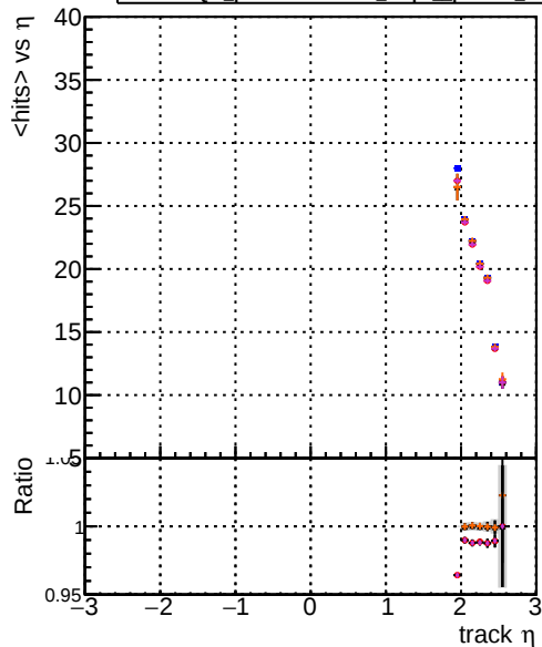
DOM original step2 pt1to20 eta2p0to2p5 DOM mkFit step2 pt1to20 eta2p0to2p5 DOM angle step2 pt1to20 eta2p0to2p5 DOM fast step2 pt1to20 eta2p0to2p5 DOM pixelCPEGeneric step2 pt1to20 eta2p0to2p5
