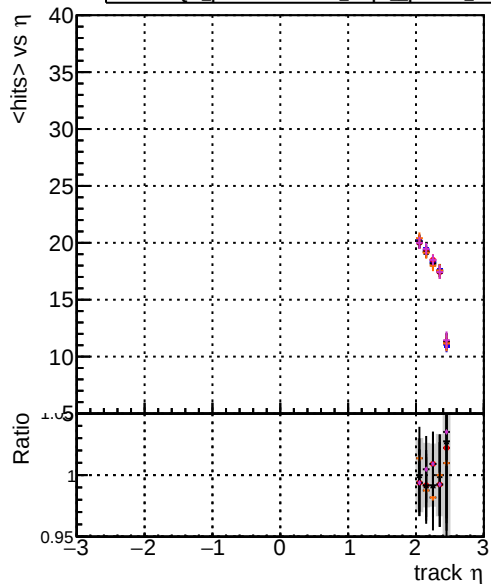
DOM original step2_pt1to20_eta2p0to2p5 DOM mkrFit_step2_pt1to20_eta2p0to2p5 DOM angle_step2_pt1to20_eta2p0to2p5 DOM fast_step2_pt1to20_eta2p0to2p5 DOM_pixelCPEGeneric_step2_pt1to20_eta2p0to2p5
