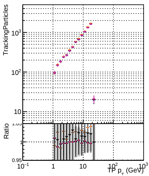
— DOM original step2 pt1to20 eta2p0to2p5 — DOM mkFit step2 pt1to20 eta2p0to2p5 — DOM angle step2 pt1to20 eta2p0to2p5 — DOM fast step2 pt1to20 eta2p0to2p5 — DOM pixelCPEGeneric step2 pt1to20 eta2p0to2p5
