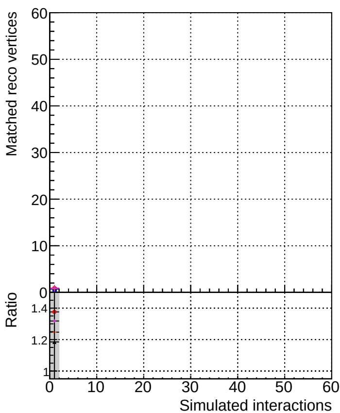
MatchedRecoVtx_vs_GenVtx
