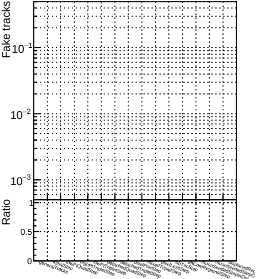
Number Color Label 1 Blue DQM original_step2_pt1to20_eta2p0to2p5 2 Red DQM cut_step2_pt1to20_eta2p0to2p5 3 Green DQM angle_step2_pt1to20_eta2p0to2p5 4 Orange DQM fast_step2_pt1to20_eta2p0to2p5 5 Purple DQM pixelCPEgeneric_step2_pt1to20_eta2p0to2p5
