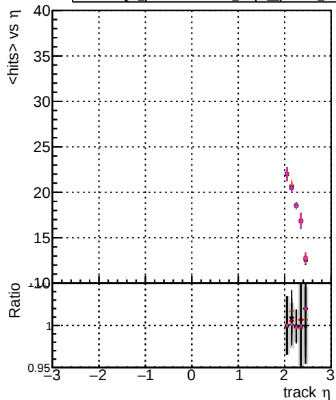
DOM original step2 pt1to20 eta2p0to2p5 DOM mkFit step2 pt1to20 eta2p0to2p5 DOM angle step2 pt1to20 eta2p0to2p5 DOM fast step2 pt1to20 eta2p0to2p5 DOM pixelCPEGeneric step2 pt1to20 eta2p0to2p5
