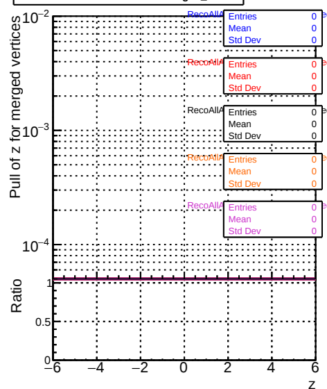
RecoAllAssoc2GenMatchedMerged_PullZ
