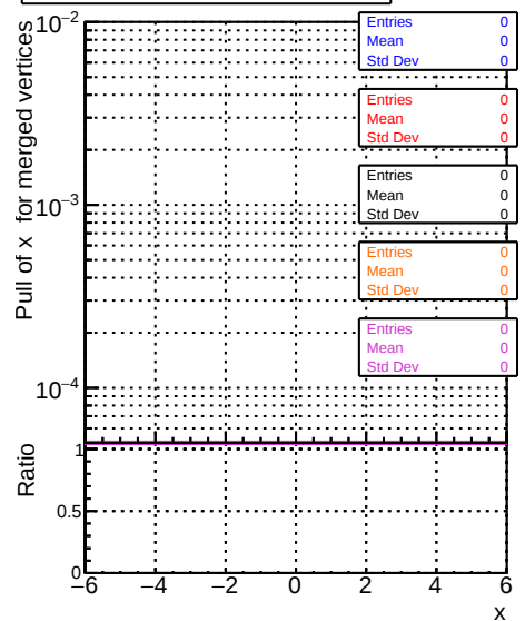
RecoAllAssoc2GenMatchedMerged_PullX
