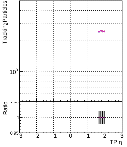
— DQM original step2_pt1to20_eta1p6to2p0 — DQM mkFit_step2_pt1to20_eta1p6to2p0 — DQM angle_step2_pt1to20_eta1p6to2p0 — DQM fast_step2_pt1to20_eta1p6to2p0 — DQM pixelCPEGeneric_step2_pt1to20_eta1p6to2p0
