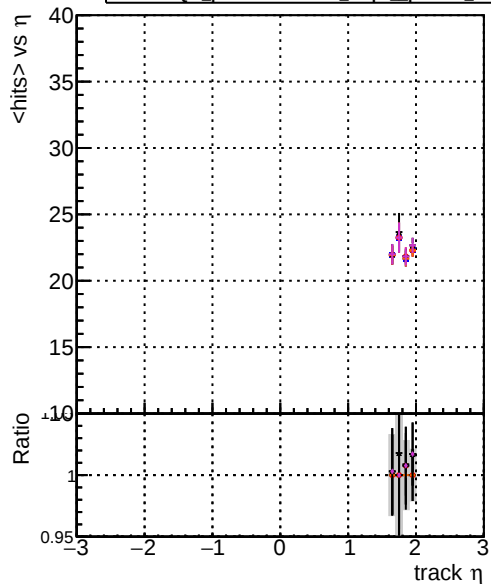
DOM original step2_pt1to20_eta1p6to2p0 DOM mkrfit_step2_pt1to20_eta1p6to2p0 DOM angle_step2_pt1to20_eta1p6to2p0 DOM fast_step2_pt1to20_eta1p6to2p0 DOM_pixelCPEGeneric_step2_pt1to20_eta1p6to2p0
