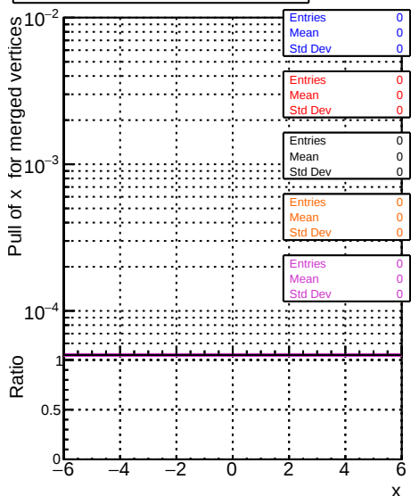
RecoAllAssoc2GenMatchedMerged_PullX
