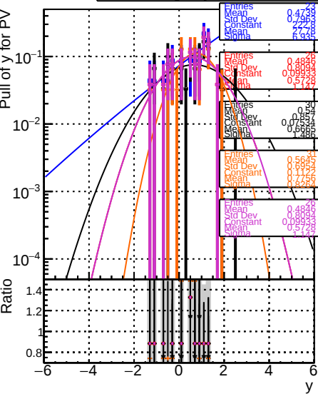
RecoPVAssoc2GenPVMatched_PullY Legend: original_step2_pt1to20_eta1p6to2p0 single_step2_pt1to20_eta1p6to2p0 fixed_PEGeneric_step2_pt1to20_eta1p6to2p0
