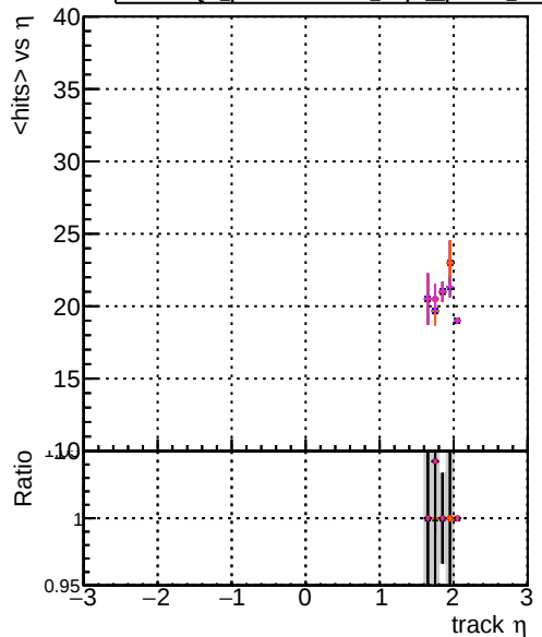
DOM original step2 pt1to20 eta1p6to2p0 DOM mkFit step2 pt1to20 eta1p6to2p0 DOM angle step2 pt1to20 eta1p6to2p0 DOM fast step2 pt1to20 eta1p6to2p0 DOM pixelCPEGeneric step2 pt1to20 eta1p6to2p0
