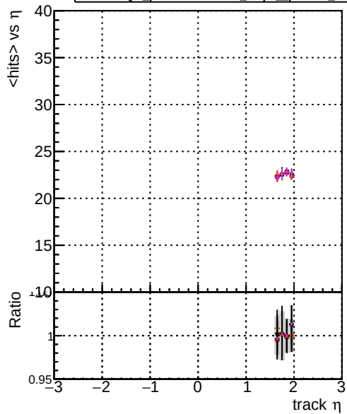
DOM original step2 pt1to20 eta1p6to2p0 DOM mkrFit step2 pt1to20 eta1p6to2p0 DOM angle step2 pt1to20 eta1p6to2p0 DOM fast step2 pt1to20 eta1p6to2p0 DOM pixelCPEGeneric step2 pt1to20 eta1p6to2p0
