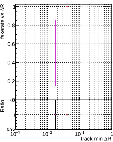
Fake rate vs \Delta R(\text{track}, \text{jet}) DQM original step2 pt1to20 eta1p6to2p0 DQM angle step2 pt1to20 eta1p6to2p0 DQM angle step2 pt1to20 eta1p6to2p0 DQM fixerCPGeneric step2 pt1to20 eta1p6to2p0
