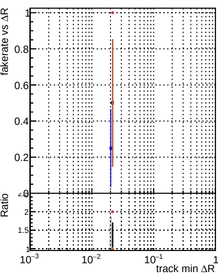
Fake rate vs ΔR(track, jet) Legend: DOM (blue line with dots) original_step2_pt1to20_eta1p6to2p0 (orange line with dots) angle_step2_pt1to20_eta1p6to2p0 (red line with dots) PixelCPEGeneric_step2_pt1to20_eta1p6to2p0 (green line with dots)
