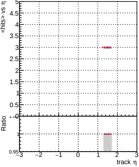
mean hit DOM original step2_pt1to20_eta1p4to1p6 DOM mkrFit_step2_pt1to20_eta1p4to1p6 DOM angle_step2_pt1to20_eta1p4to1p6 DOM fast_step2_pt1to20_eta1p4to1p6 DOM pixelCPEGeneric_step2_pt1to20_eta1p4to1p6
