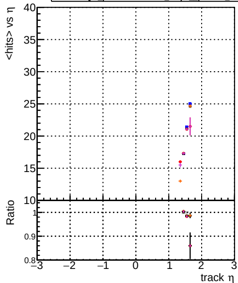
mean hit DOM original step2_pt1to20_eta1p4to1p6 DOM mkFit_step2_pt1to20_eta1p4to1p6 DOM angle step2_pt1to20_eta1p4to1p6 DOM fast step2_pt1to20_eta1p4to1p6 DOM pixelCPEGeneric step2_pt1to20_eta1p4to1p6
