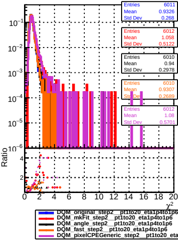
normalized \chi^2
