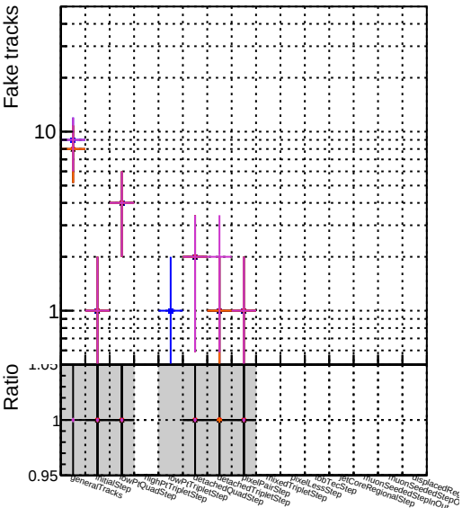
Number DOM angle step2 p1to1000 eta2p0to2p5 DOM fast step2 p1to1000 eta2p0to2p5 DOM pixelCPEGeneric step2 p1to1000 eta2p0to2p5
