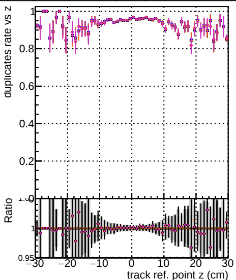
—●— DOM original step2 pt1to1000 eta2p0to2p5 —●— DOM original step2 pt1to1000 eta2p0to2p5 —●— DOM original step2 pt1to1000 eta2p0to2p5 —●— DOM original step2 pt1to1000 eta2p0to2p5
