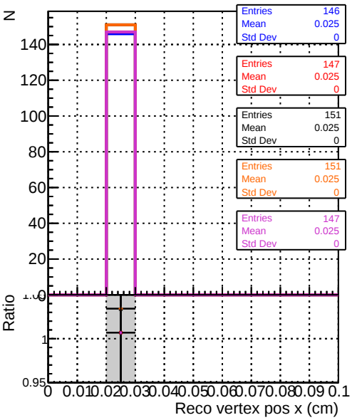
Recons DOM original step2 pt1to1000 eta2p0to2p5 DOM mkFit step2 pt1to1000 eta2p0to2p5 DOM angle step2 pt1to1000 eta2p0to2p5 DOM fast step2 pt1to1000 eta2p0to2p5 DOM pixelCPEGeneric step2 pt1to1000 eta2p0to2p5
