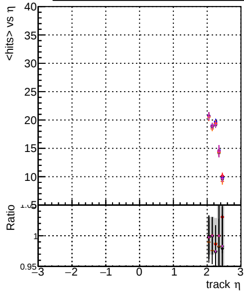
DOM original step2 p_t1to1000 eta2p0to2p5 DOM mkrFit_step2 p_t1to1000 eta2p0to2p5 DOM angle_step2 p_t1to1000 eta2p0to2p5 DOM fast_step2 p_t1to1000 eta2p0to2p5 DOM pixelCPEGeneric_step2 p_t1to1000 eta2p0to2p5
