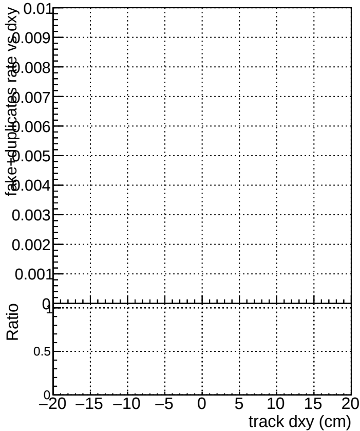
DQM original step2_pt1to1000_eta2p0to2p5 DQM mkFit_step2_pt1to1000_eta2p0to2p5 DQM angle_step2_pt1to1000_eta2p0to2p5 DQM fast_step2_pt1to1000_eta2p0to2p5 DQM pixelCPEGeneric_step2_pt1to1000_eta2p0to2p5
