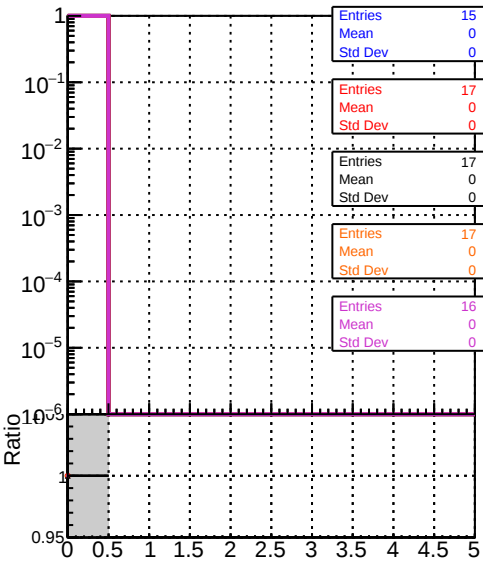
mean hits vs \eta DOM original step2_pt1to1000_eta2p0to2p5 DOM mkFit_step2_pt1to1000_eta2p0to2p5 DOM angle_step2_pt1to1000_eta2p0to2p5 DOM fast_step2_pt1to1000_eta2p0to2p5 DOM pixelCPEGeneric_step2_pt1to1000_eta2p0to2p5
