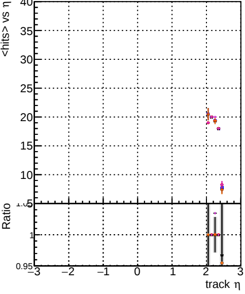
mean hits vs \eta DOM original step2_pt1to1000_eta2p0to2p5 DOM mkFit_step2_pt1to1000_eta2p0to2p5 DOM angle_step2_pt1to1000_eta2p0to2p5 DOM fast_step2_pt1to1000_eta2p0to2p5 DOM pixelCPEGeneric_step2_pt1to1000_eta2p0to2p5
