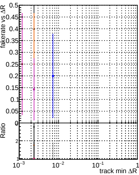
Fake rate vs ΔR(track, jet) for different methods and parameters.
