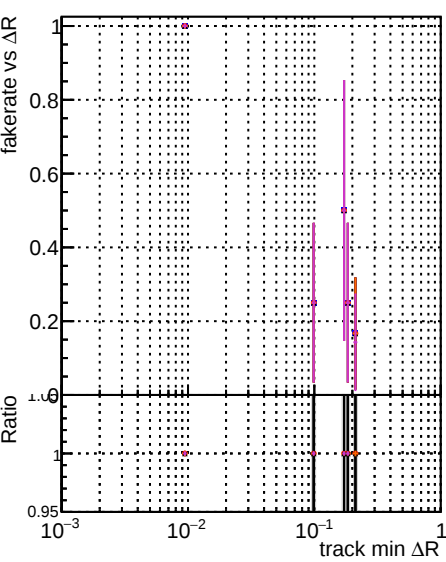
Fake rate vs \Delta R(\text{track}, \text{jet}) DQM original step2 pt1to1000 eta2p0to2p5 DQM original step2 pt1to1000 eta2p0to2p5 DQM original step2 pt1to1000 eta2p0to2p5 DQM original step2 pt1to1000 eta2p0to2p5
