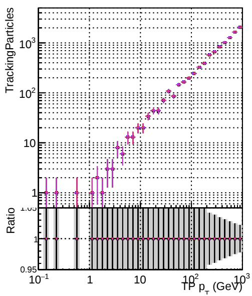
—•— DQM original step2 pt1to1000 eta2p0to2p5 —•— DQM mkFit step2 pt1to1000 eta2p0to2p5 —•— DQM angle step2 pt1to1000 eta2p0to2p5 —•— DQM fast step2 pt1to1000 eta2p0to2p5 —•— DQM pixelCPEGeneric step2 pt1to1000 eta2p0to2p5
