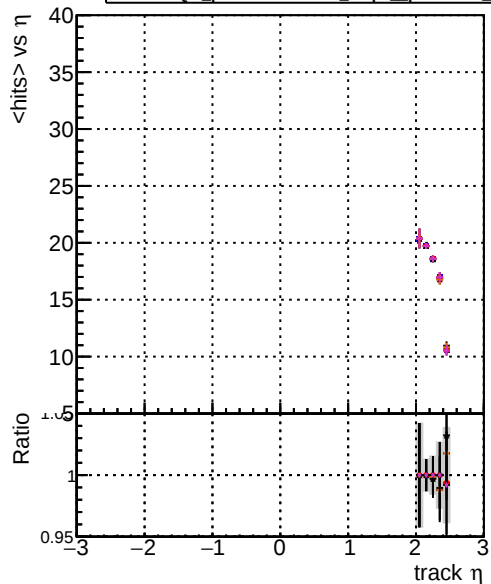
DOM original step2 p1to1000 eta2p0to2p5 DOM mkrfit step2 p1to1000 eta2p0to2p5 DOM angle step2 p1to1000 eta2p0to2p5 DOM fast step2 p1to1000 eta2p0to2p5 DOM pixelCPEGeneric step2 p1to1000 eta2p0to2p5
