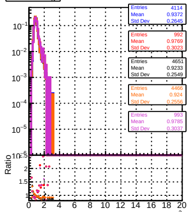
normalized \chi^2
