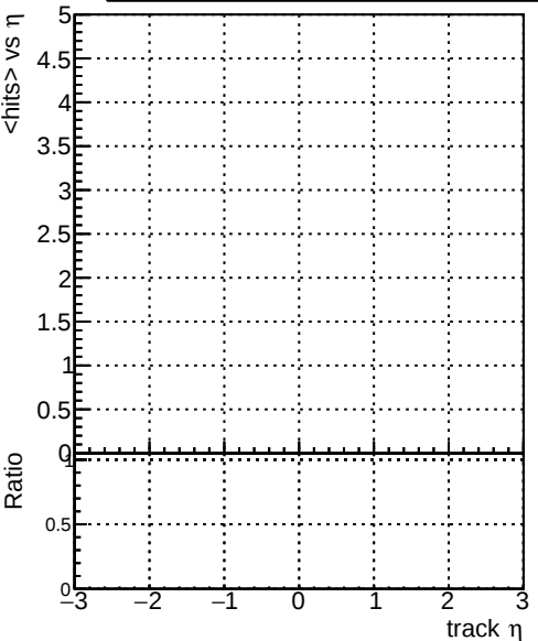
mean hit DOM_original_step2_pt1000_eta2p0to2p5 DOM_mkFit_step2_pt1000_eta2p0to2p5 DOM_angle_step2_pt1000_eta2p0to2p5 DOM_fast_step2_pt1000_eta2p0to2p5 DOM_pixelCPEGeneric_step2_pt1000_eta2p0to2p5
