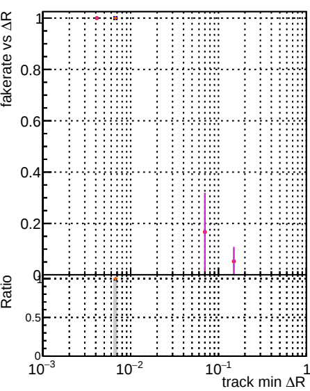
Fake rate vs ΔR(track, jet) Legend: original (blue) step2 (orange) pt1000 (green) eta2p0to2p5 (red) fixedCPGeneric (purple)
