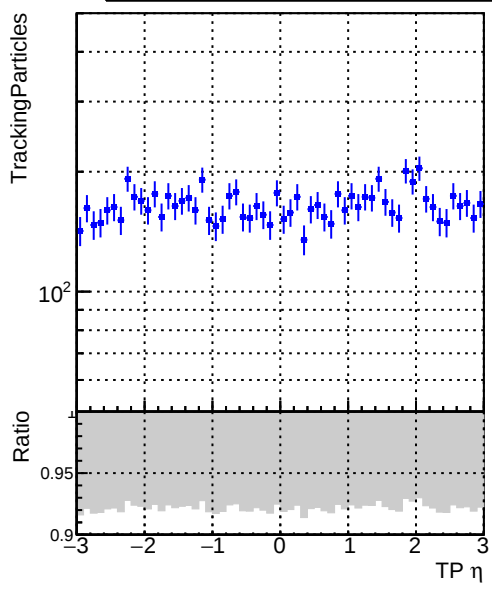
N of simulated tracks vs TP \eta Legend: DQM_V0001_R000000001_Global_CMSSW_X_Y_Z_RECO
