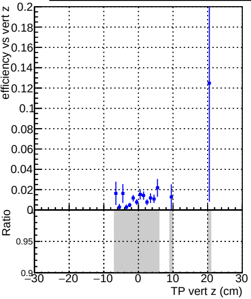
Efficiency vs vert z Legend: DQM_V0001_R000000001_Global_CMSSW_X.Y.Z_RECO
