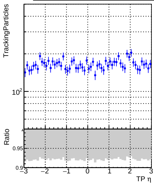
N of simulated tracks vs TP \eta Legend: DQM_V0001_R0000000001_Global_CMSSW_X.Y.Z_RECO
