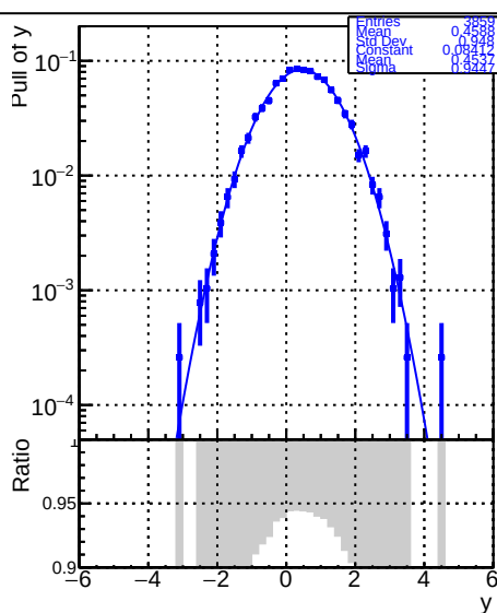
RecoPVAssoc DQM_V0001_R000000001_Global_CMSSW_X_Y_Z_RECO
