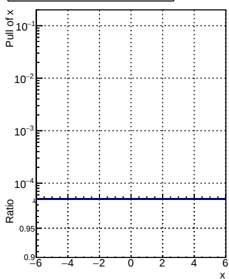
RecoAllAssoc2GenMatched_PullX
