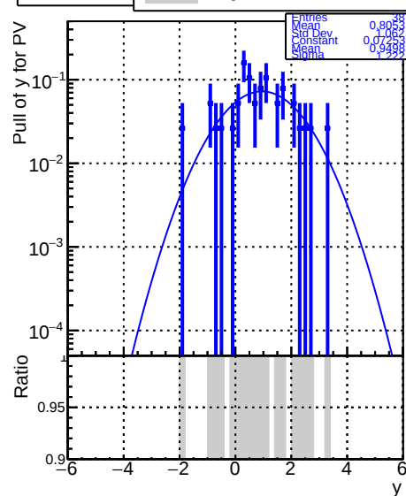
RecoPVAssoc DQM_V0001_R000000001_Global_CMSSW_X_Y_Z_RECO
