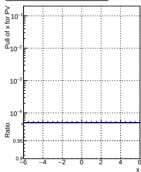
RecoPVAssoc2GenPVMatched_PullX
