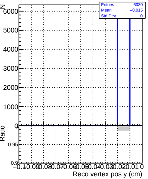
Recons DQM_V0001_R000000001_Global_CMSSW_X.Y.Z_RECO
