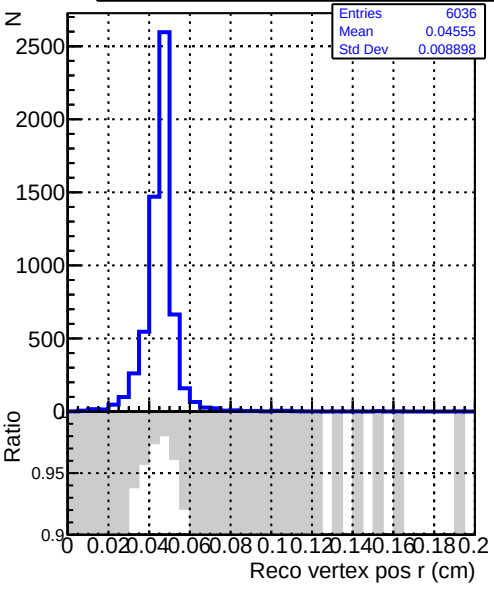
Recons DQM_V0001_R000000001_Global_CMSSW_X.Y.Z_RECO
