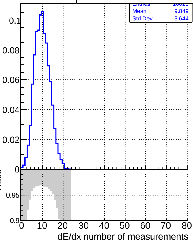
DQM_V0001_R000000001_Global_CMSSW_X_Y_Z_RECO
