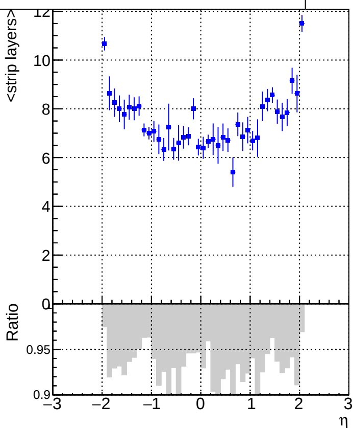
DQM_V0001_R000000001_Global_CMSSW_X_Y_Z_RECO
