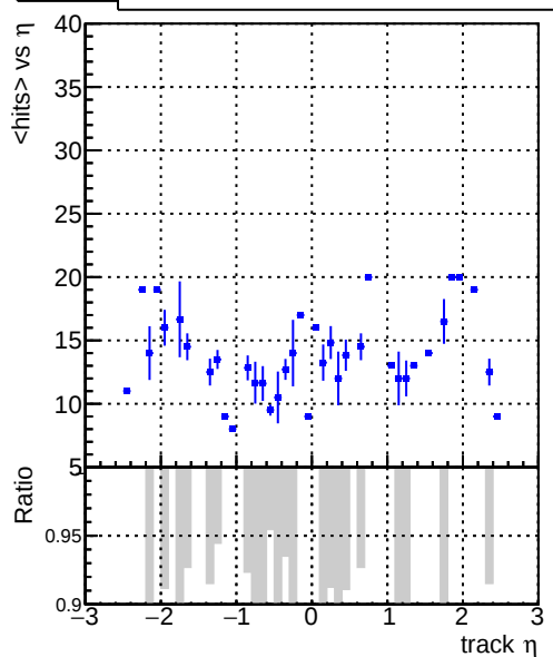
mean hits
