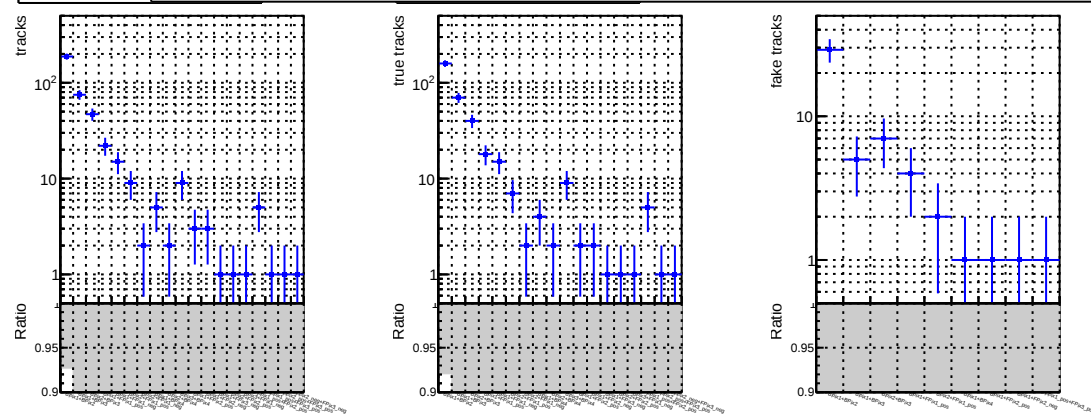
N of reco track vs. \chi^2 DQM_V0001_R000000001_Global_CMSSW_X_Y_Z_RECO
