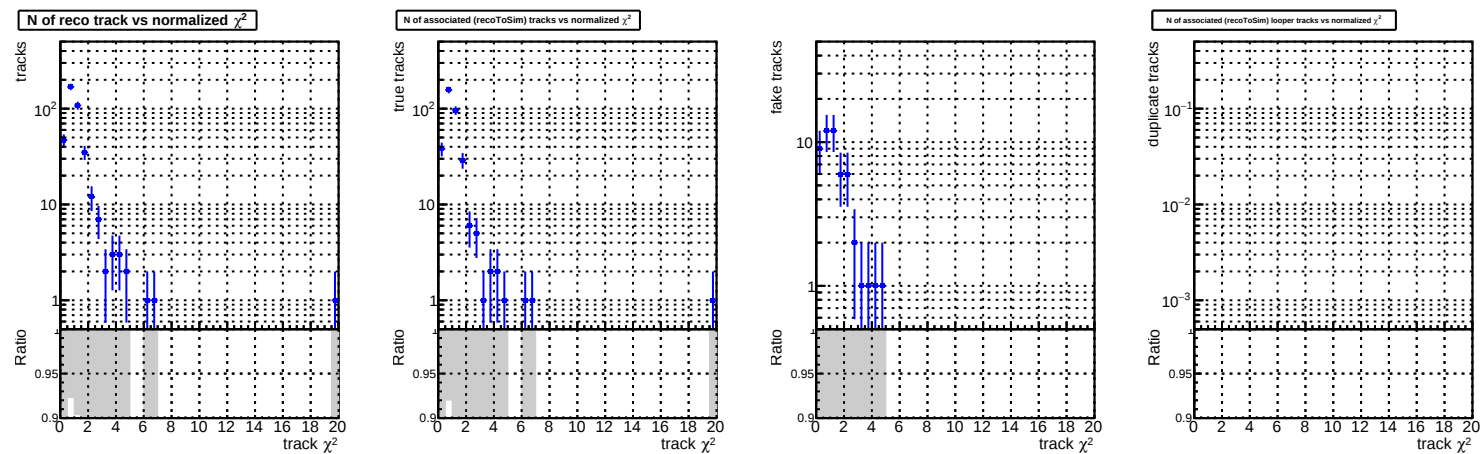
N of reco track vs. \chi^2 DQM_V0001_R000000001_Global_CMSSW_X_Y_Z_RECO
