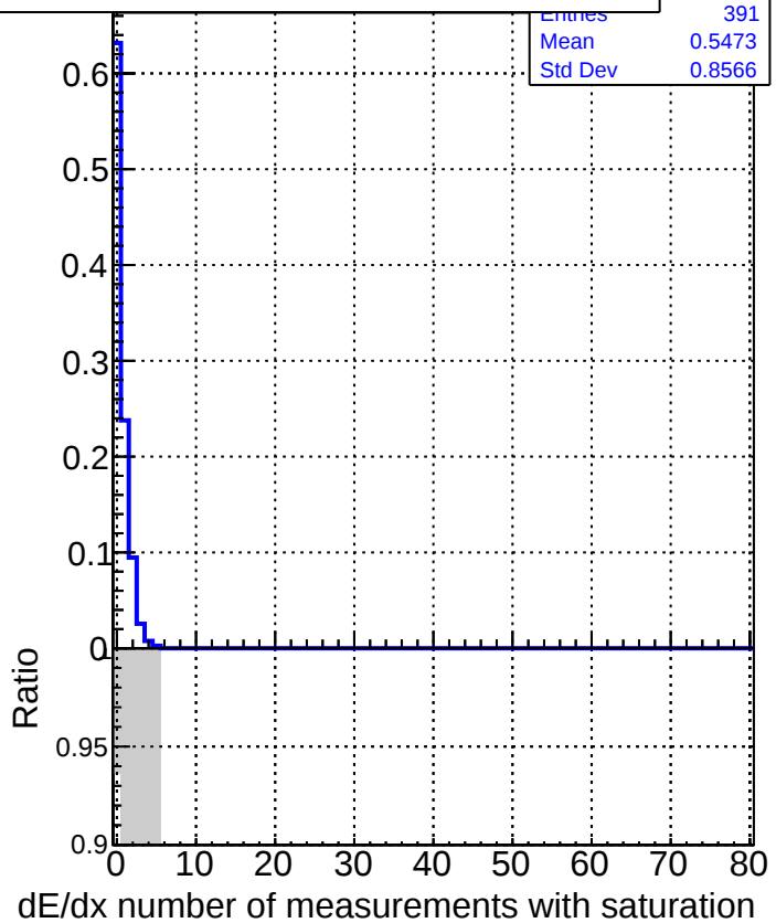
DQM_V0001_R000000001_Global_CMSSW_X_Y_Z_RECO
