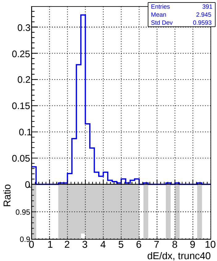
DQM_V0001_R000000001_Global_CMSSW_X_Y_Z_RECO
