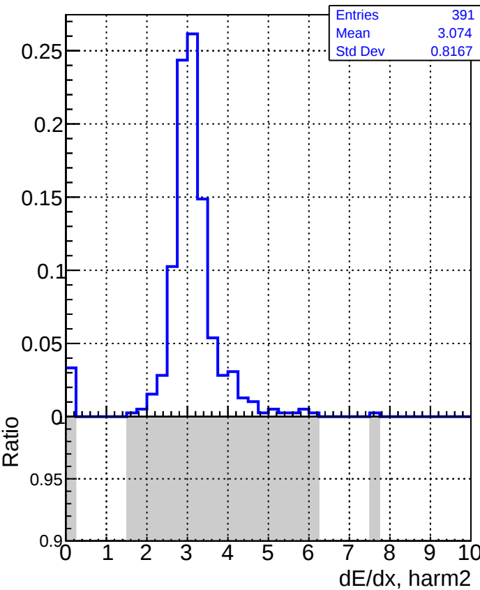
DQM_V0001_R000000001_Global_CMSSW_X_Y_Z_RECO
