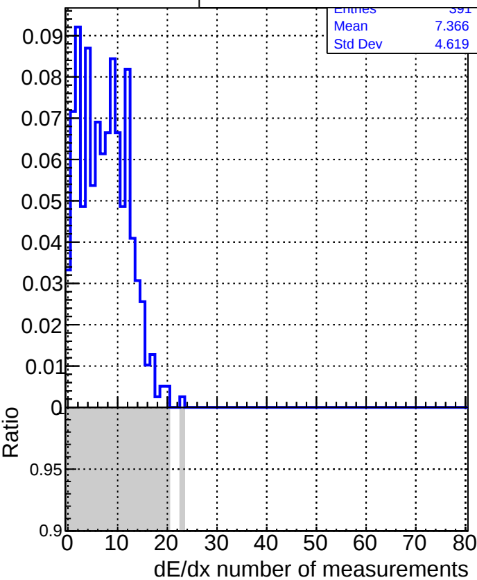
DQM_V0001_R000000001_Global_CMSSW_X_Y_Z_RECO
