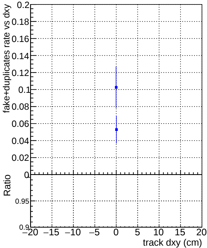
DQM_V0001_R0000000001_Global_CMSSW_X_Y_Z_RECO
