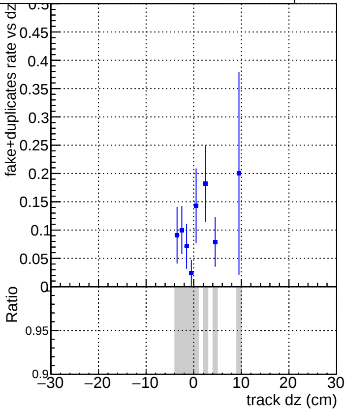
DQM_V0001_R0000000001_Global_CMSSW_X_Y_Z_RECO
