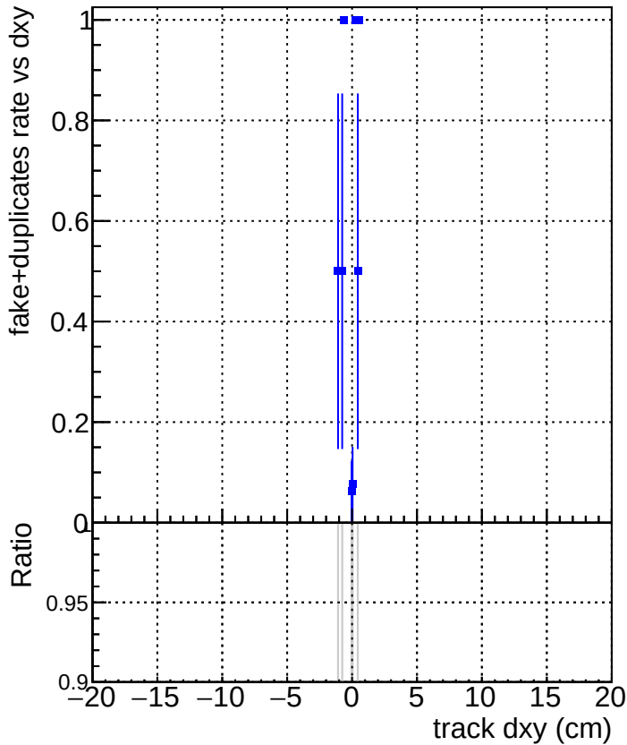
DQM_V0001_R000000001_Global_CMSSW_X_Y_Z_RECO
