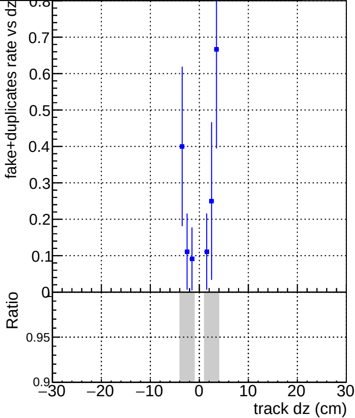
DQM_V0001_R000000001_Global_CMSSW_X_Y_Z_RECO
