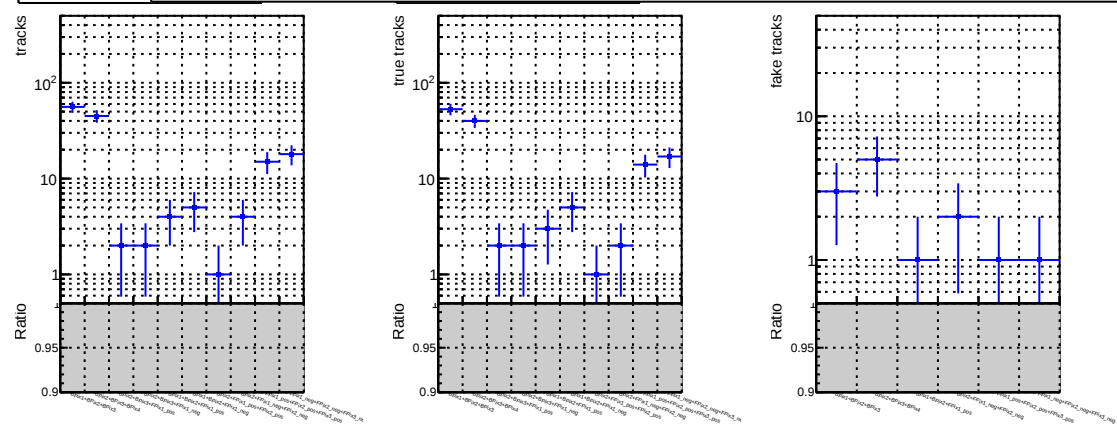
N of reco track vs. \chi^2 —●— DQM_V0001_R000000001_Global_CMSSW_X_Y_Z_RECO
