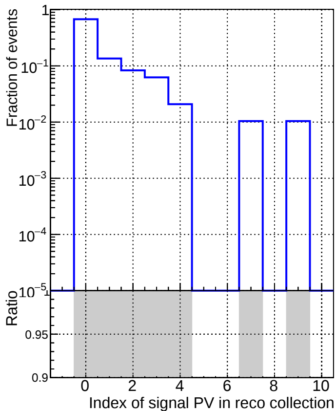
DQM_V0001_R000000001_Global_CMSSW_X_Y_Z_RECO
